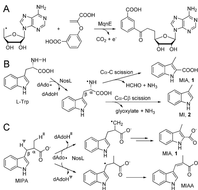
Figure 1. Reactions catalyzed by the radical SAM enzymes MqnE and NosL. A) The MqnE-catalyzed dAdo radical-based addition reaction involved in menaquinone biosynthesis. B) The NosL-catalyzed promiscuous reactions with the authentic substrate L-Trp. C) Two routes of hydrogen abstraction in NosL reaction with an unnatural substrate MIPA. The two hydrogens abstracted by the dAdo radical are shown by triangles and rectangles, respectively.
