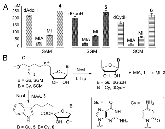
Figure 3. NosL acts on two SAM analogues SGM and SCM. A) The yields of different products in NosL reaction with SAM, SGM, or SCM. Assays were carried out by incubating 500 \mu\text{M} substrates (L-Trp or IMAA, 3 ) with 50 \mu\text{M} reconstituted protein, 500 \mu\text{M} SAM, and 2 mM of sodium dithionite in 50 mM MOPS buffer (pH 8.0) for 1.5 h. Assays were performed in duplicates, and the standard deviations (S.D.) are shown by the error bars. B) Two types of reactions (hydrogen abstraction and radical addition) catalyzed by NosL with the SAM analogues.
