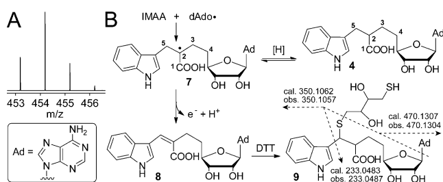
Figure 4. Mechanistic insights into the NosL-catalyzed dAdo radical-based addition reaction. A) The mass spectrum of 4 produced in the NosL reaction with IMAA in D 2 O buffer (pD 8.0, 90% D 2 O). The spectrum clearly shows that 4 is mainly mono-deuterated and partially di-deuterated. B) Divergence of the radical intermediate 7 into two reaction pathways, producing the reduced product 4 and the desaturated product 8 , the latter is further converted to a DTT adduct 9 by Michael addition of DTT to 8 . Part of the collision-induced dissociation (CID) ion fragments of 9 was shown, and the full HR-MS/MS spectrum of 9 and 8 were shown in Figures S11B and S12B, respectively.
