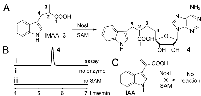
Figure 2. Investigation of NosL reaction by using L-Trp analogues. A) NosL-catalyzed reaction with IMAA 3 , which produces an adenosine adduct 4 . B) LC-MS analysis of the IMAA reaction mixture, showing the extracted ion chromatograms (EICs) of [M+H]^+ = 453.2 (corresponding to 4 ) for i) NosL-catalyzed reaction with all the required components, ii) control reaction with boiled NosL, and iii) control reaction in which SAM was omitted. C) NosL does not act on IMAA analogue 2-(indolyl)acrylic acid (IAA).
